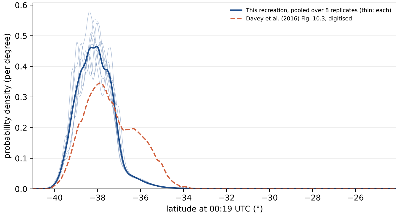
Latitude pdf at 00:19 UTC — tempered-three
